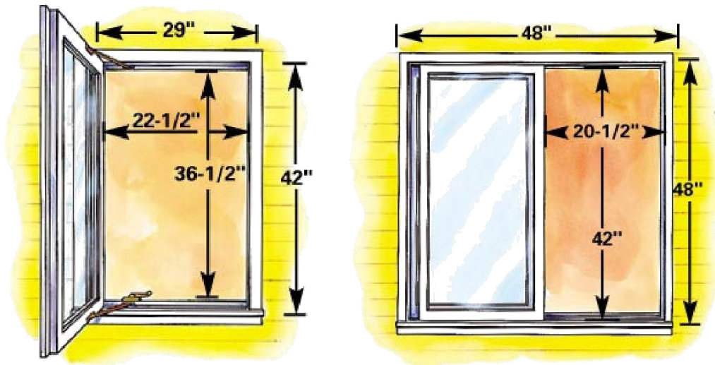
Note: Dimensions shown only for illustration purposes
